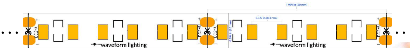
(This drawing is an excerpt that shows just two complete, cuttable sections. Each reel consists of 100 of these sections).
